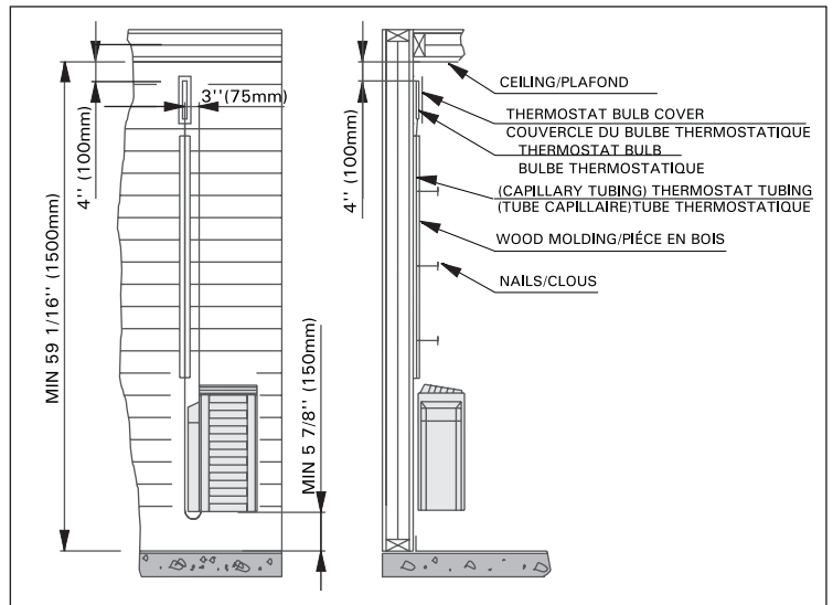
Figure 7. Installation of the thermostat sensor
